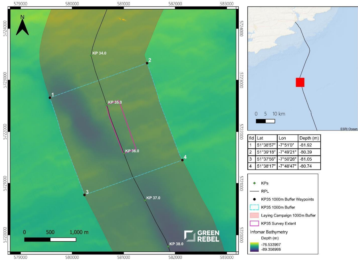
Figure 1: Cable Repair Area Buffer and Coordinates at KP35
